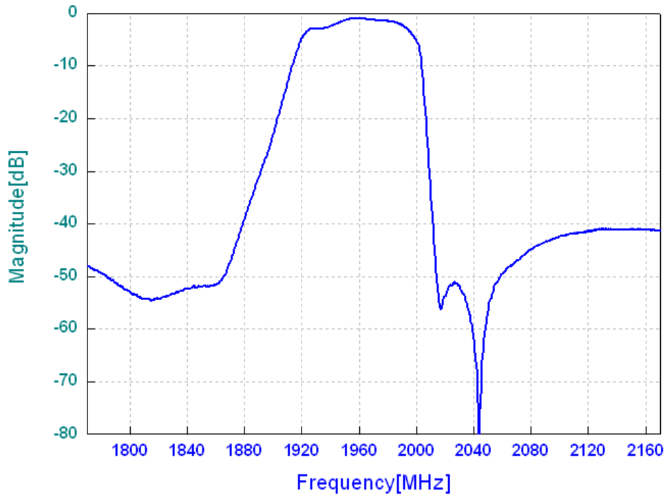
Frequency Response
